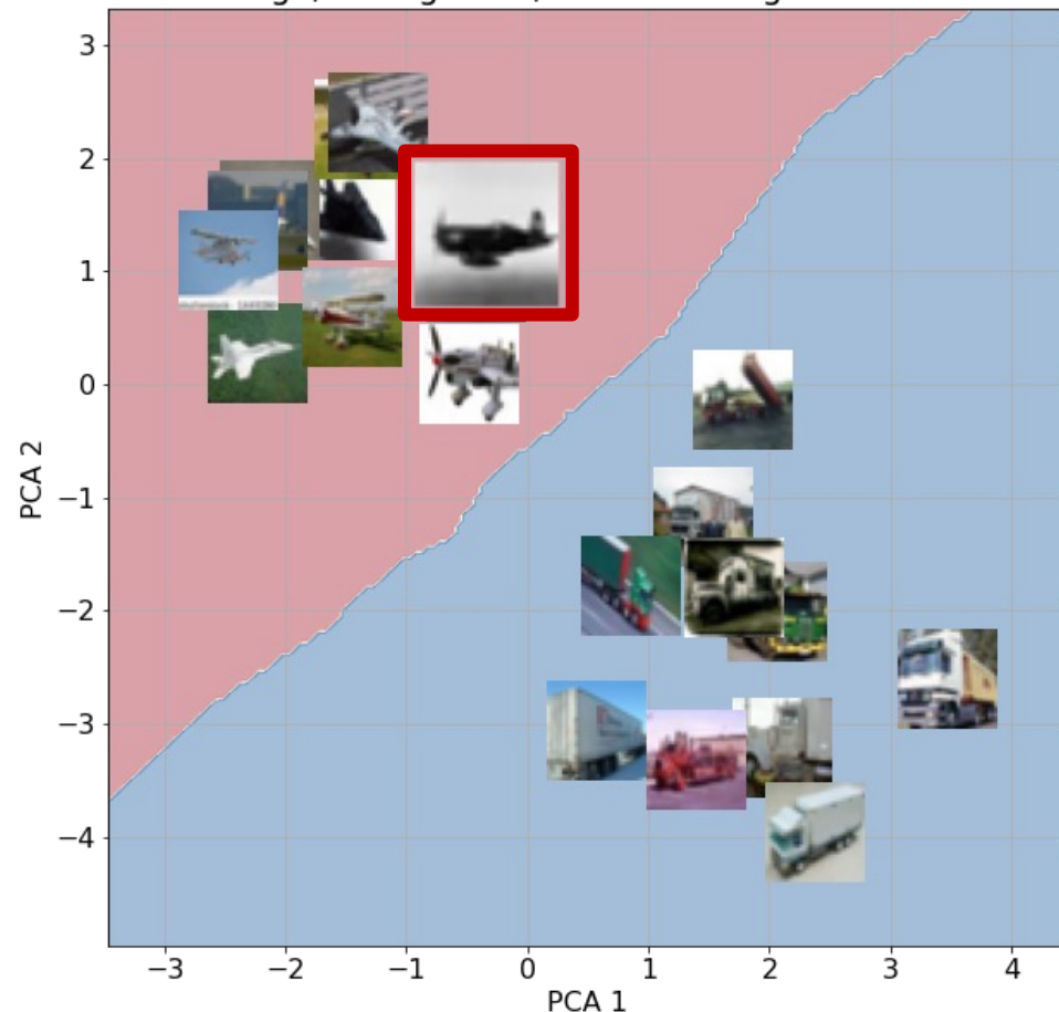
KNN Example (K=3) - CIFAR-10 Images in 2D PCA Space Test Image, 3 Neighbors, and KNN Neighborhood Circle
