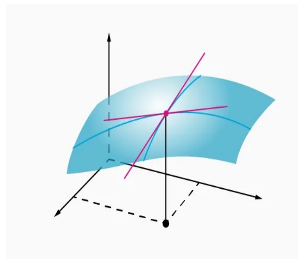
\nabla f(x, y)
